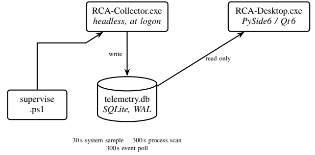
Fig. 1. Process architecture. The collector writes; the desktop application only reads. A PowerShell supervisor restarts the collector without needing administrator rights.
