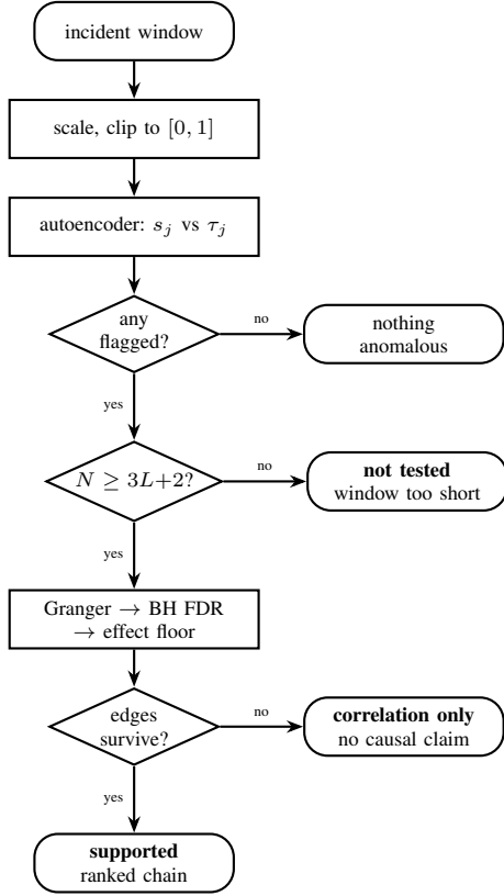
Fig. 2. Inference pipeline. Four end states are reported separately, so “not tested” is never shown as “nothing survived”.
