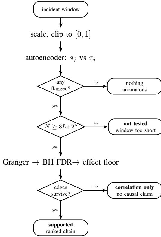
Fig. 2. Inference pipeline. Four terminal states are reported distinctly. Collapsing “not tested” into “nothing survived” would conflate the absence of a result with a negative result, which earlier revisions of this system did.
