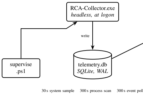
Fig. 1. Process architecture. The collector writes; the desktop application only reads. A PowerShell supervisor restarts the collector if it exits unexpectedly, because creating a Task Scheduler logon task requires elevation that a diagnostic tool should not demand.
