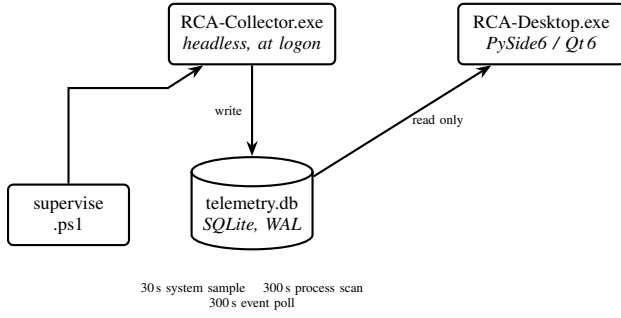
Fig. 1. Process architecture. The collector writes; the desktop application only reads. A PowerShell supervisor restarts the collector if it exits unexpectedly, because creating a Task Scheduler logon task requires elevation that a diagnostic tool should not demand.
