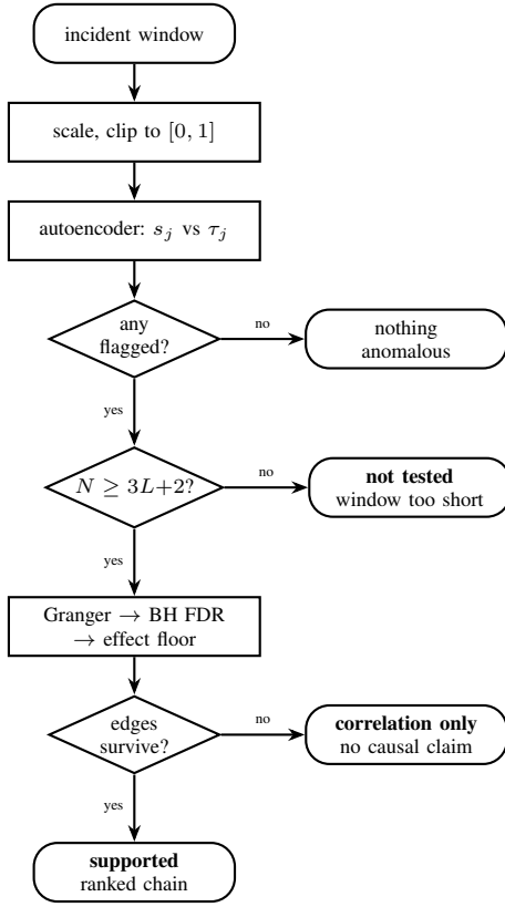
Fig. 2. Inference pipeline. Four terminal states are reported distinctly. Collapsing “not tested” into “nothing survived” would conflate the absence of a result with a negative result, which earlier revisions of this system did.
