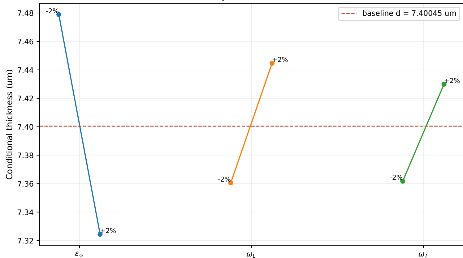
Thickness sensitivity to fixed SiC material constants
