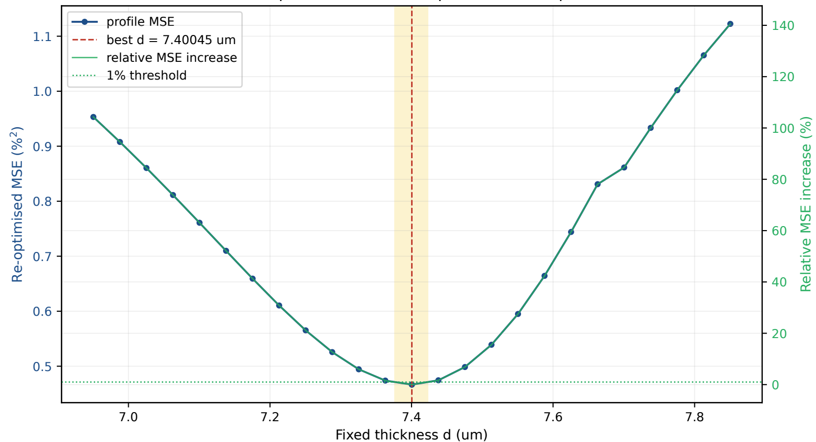
Thickness profile with nuisance parameters re-optimised
