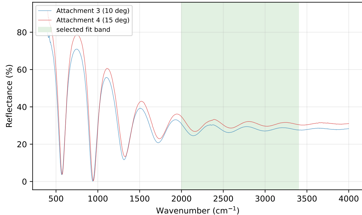
Silicon input spectra and selected common band
