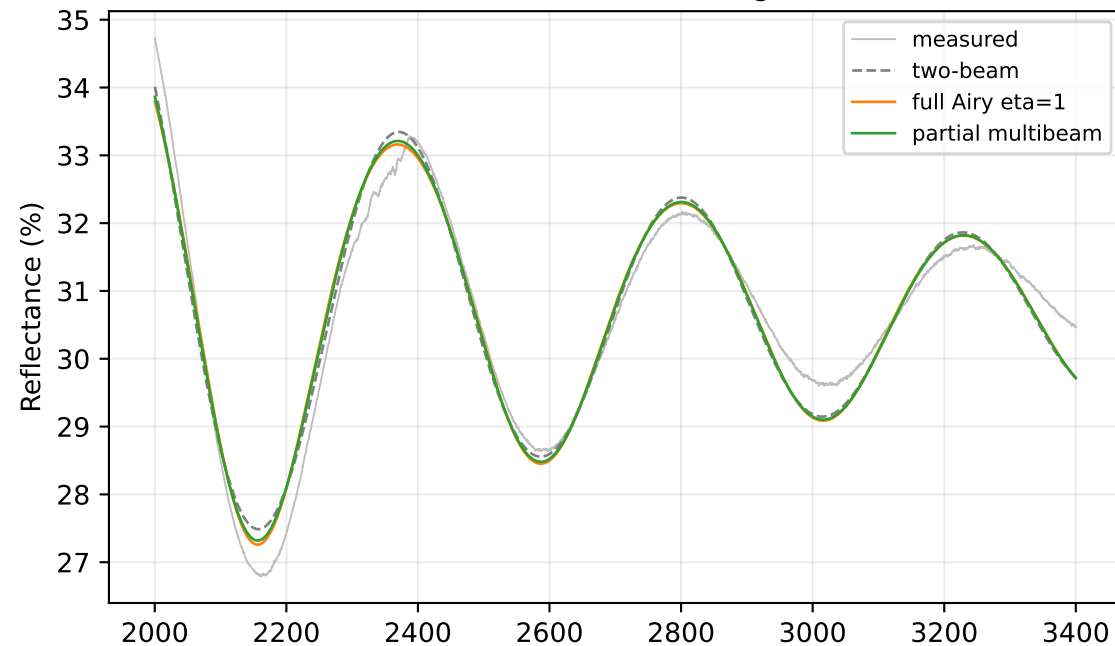
Silicon two-beam / full-Airy / partial-multibeam comparison Attachment 3 (10 deg)
