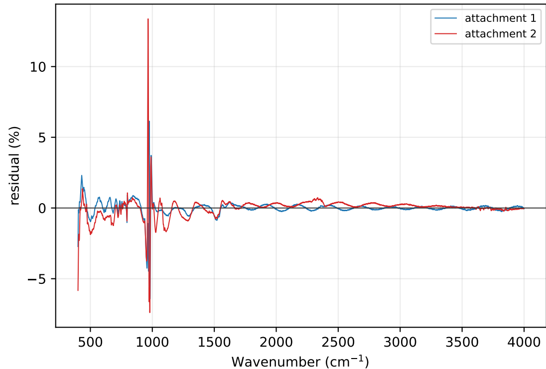
SiC correction: d 7.400452 -> 7.399476 \mu\text{m} SiC exact-Airy correction fit
