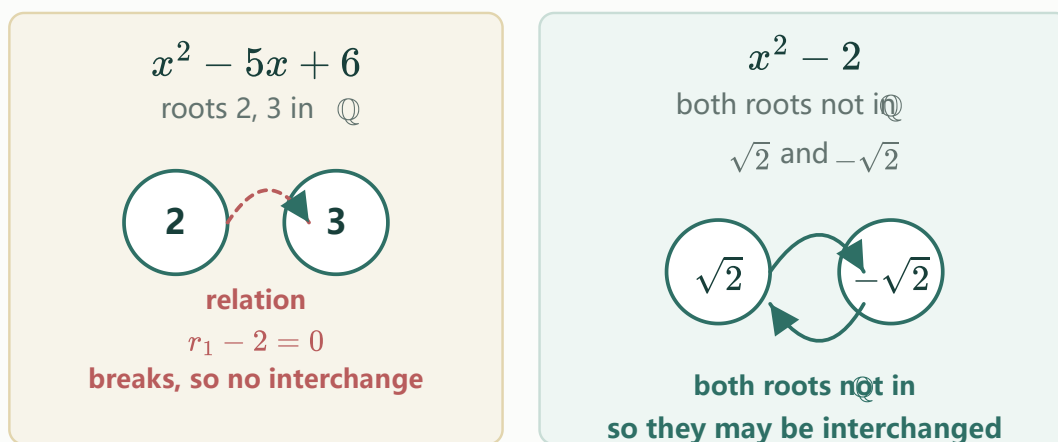
Figure 1: Vieta Symmetry vs Root Interchange
