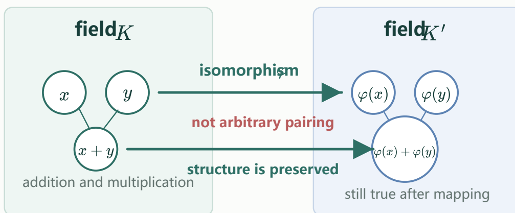
Figure 3: Isomorphism Preserves Structure
