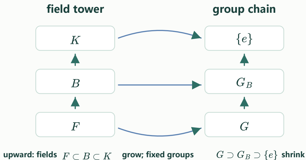
Figure 6. Moving upward in the field tower makes the field larger; the corresponding fixed group becomes smaller.
