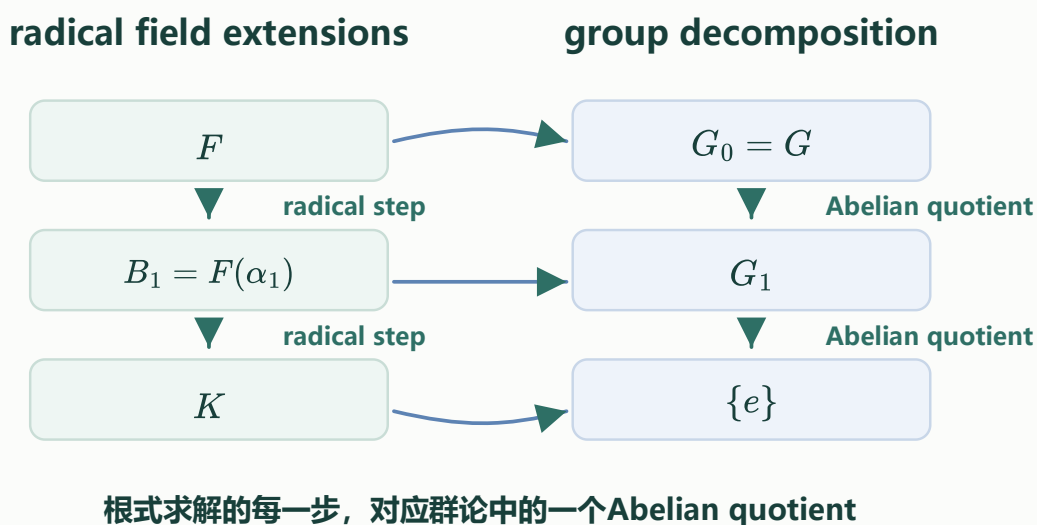
Figure 8: Radicals and Solvable Groups in Parallel
