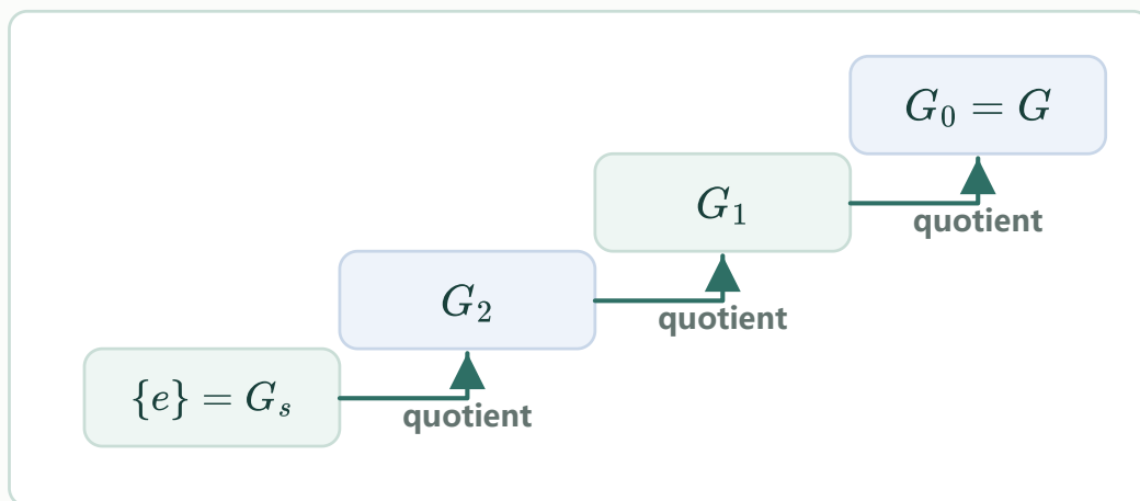
Figure 7: A Normal Subgroup Chain as a Staircase
