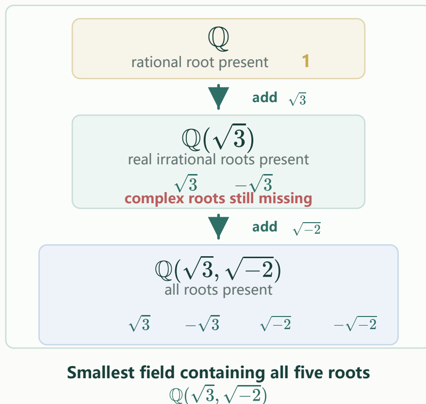
Figure 2: Splitting Field of This Quintic
