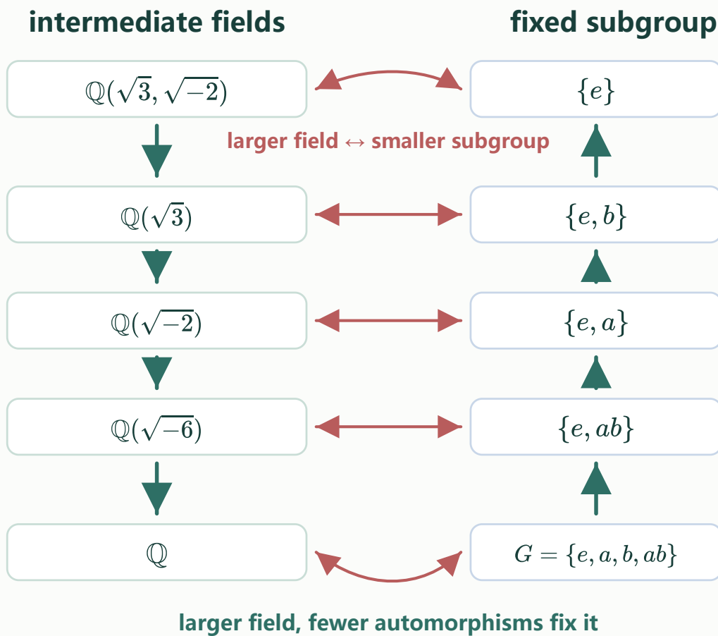
Figure 6. Larger fields correspond to smaller fixed subgroups; in this example the correspondence can be drawn explicitly.
