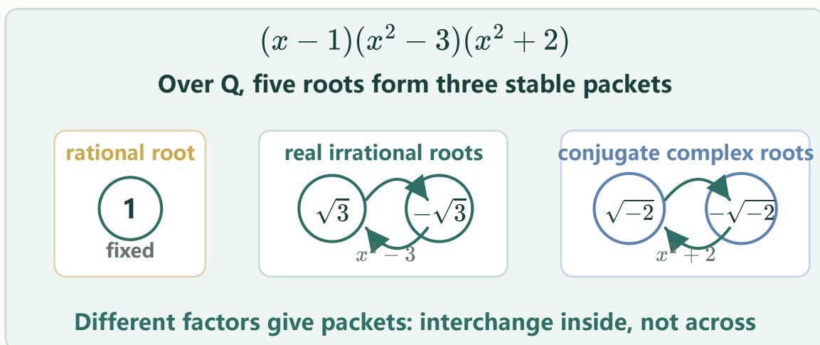
Figure 1: Three Types of Roots in One Quintic
