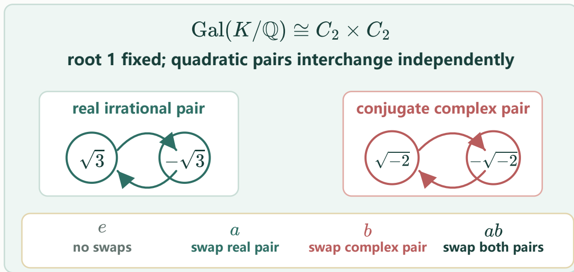
Figure 5: This Galois Group Has Four Elements
