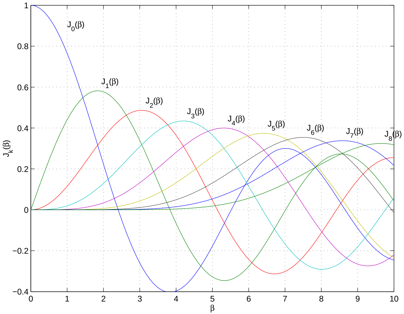
Plots of Bessel Functions of the First Kind
