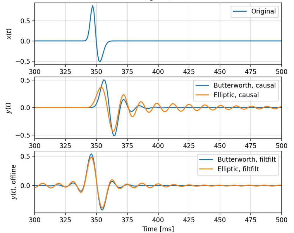
Filtered Testsignals, f_s=1000 Hz
