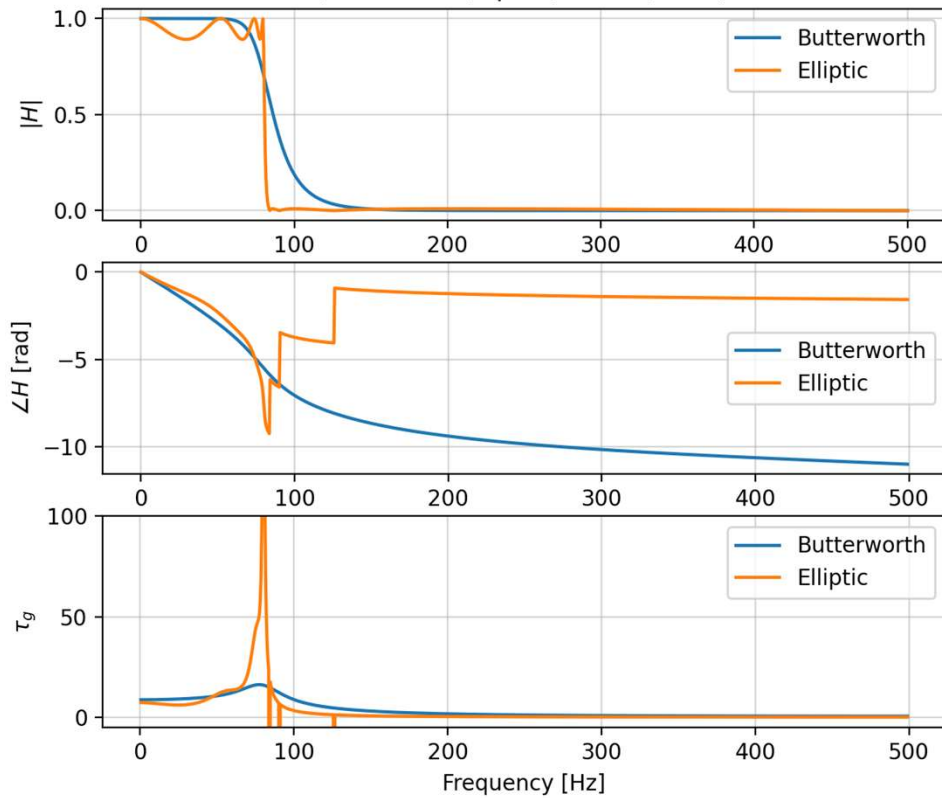
IIR Filters, w_c=80 Hz, r_p=1 , r_s=40 , N=7 , f_s=1000
