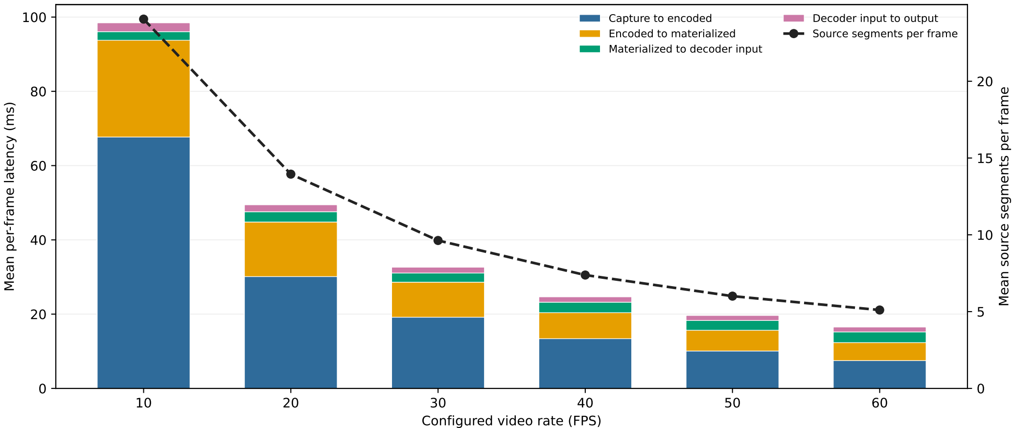
Higher FPS reduces pre-network frame work; fetch/reassembly stays flat
