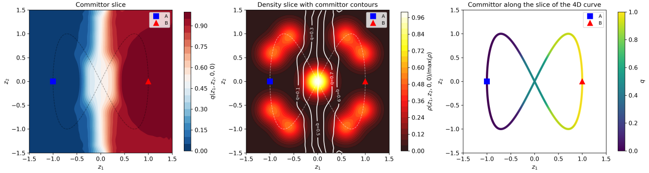
FIGURE 3. The 4 dimensional toy example with N = 10 . Qualitatively, these plots look pretty similar to the two dimensional case and so agree with what one would generally expect. We note that this result was highly sensitive to parameter selection so we hypothesize that better results can be obtained with more careful parameter tuning.
