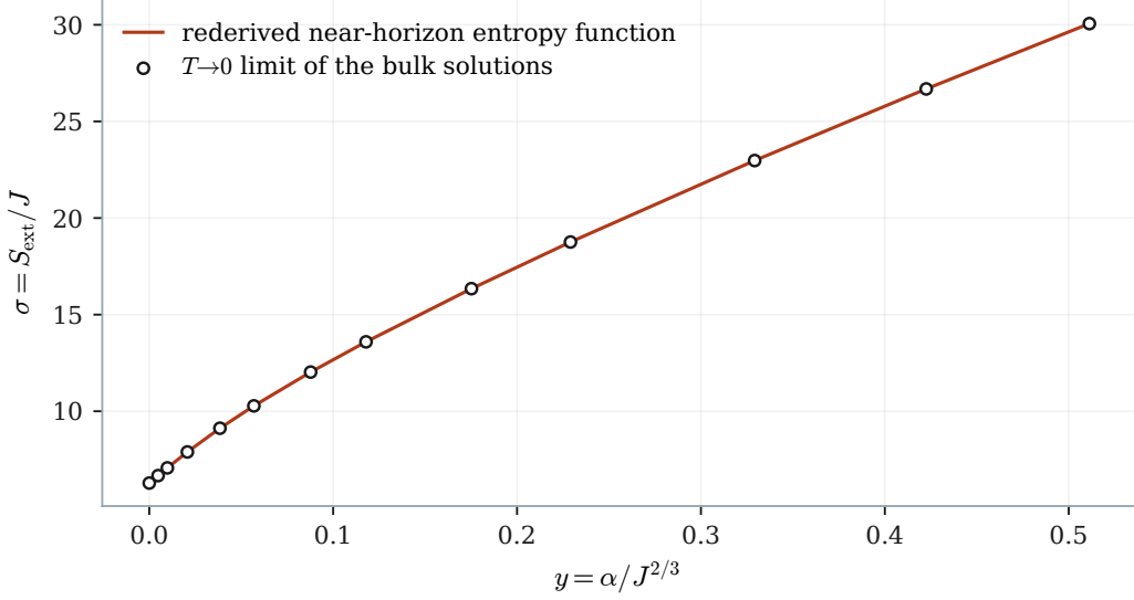
Figure 6. Extremal entropy per angular momentum. The line joins values from our rederived near-horizon entropy function, checked against the equations of [11] to the precision quoted in the text; the points are extrapolations of bulk solutions to zero temperature.
