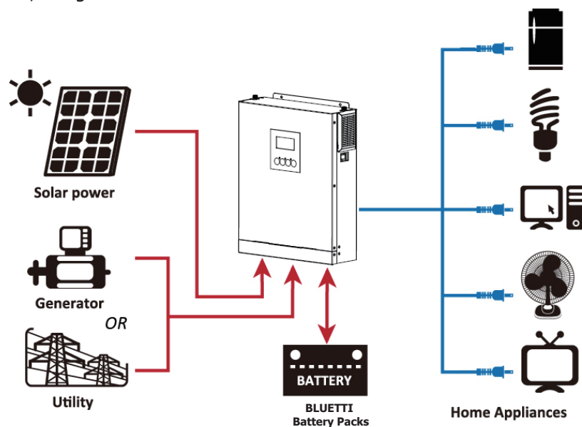
Figure 1 Solar Power System
