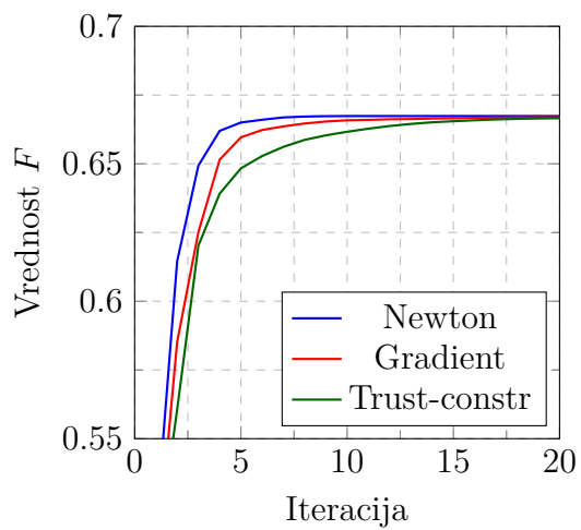
(c) n = 20 točk
