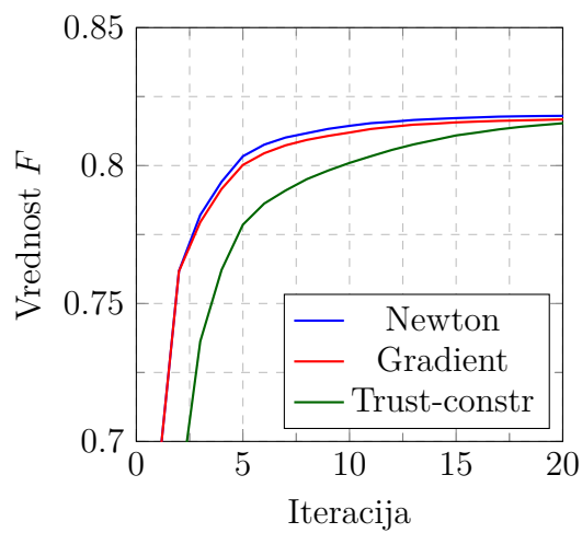
(e) n = 40 točk
