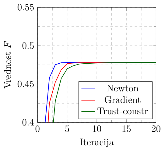
(a) n = 5 točk
