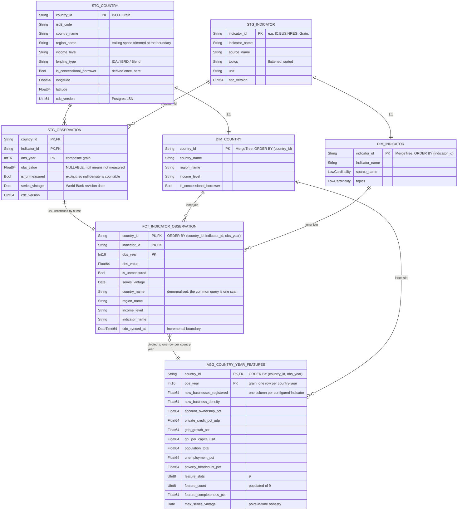
ERD. Full resolution: diagrams/exports/. Source: diagrams/src/erd.mmd
