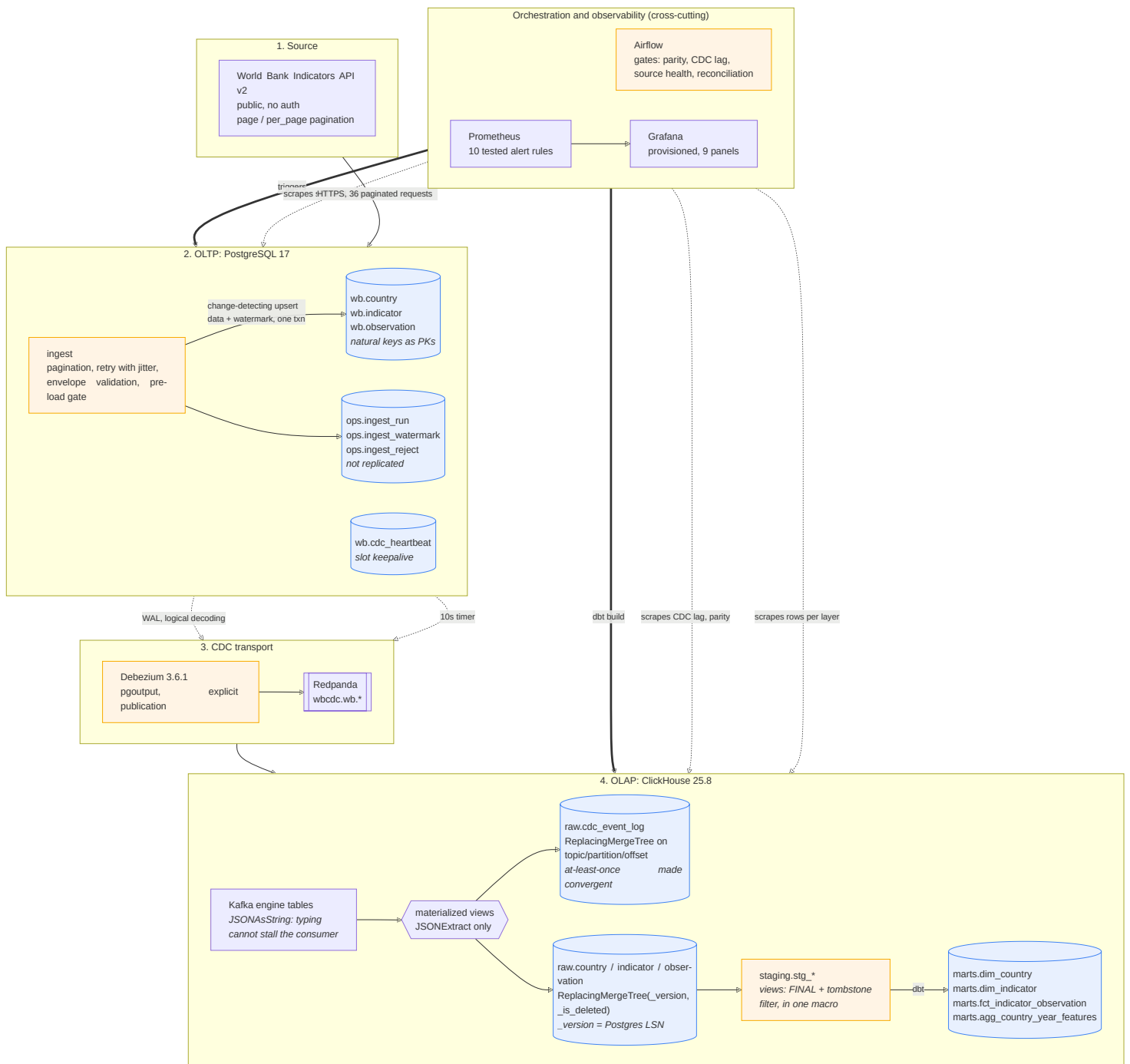
Architecture. Full resolution: diagrams/exports/. Source: diagrams/src/architecture.mmd
