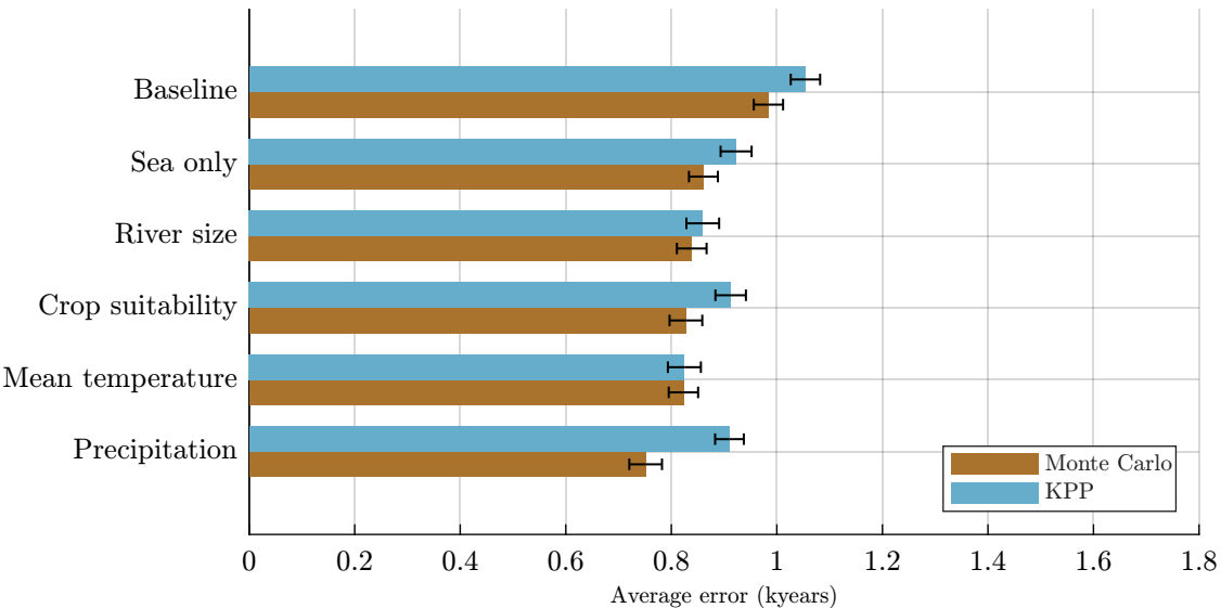
Maize: Monte Carlo vs. KPP
