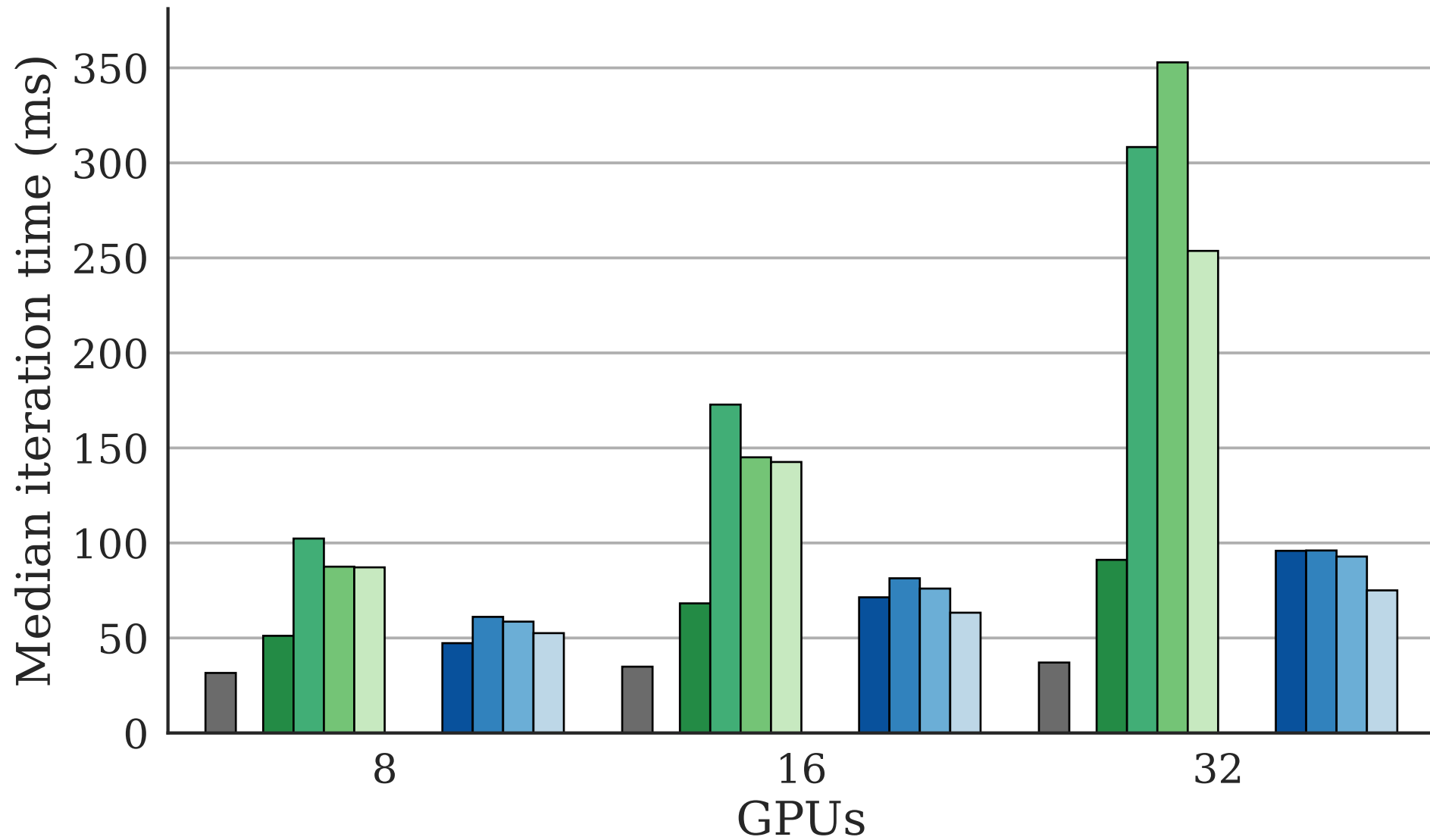
WideResNet on Frontier (AMD, MPI) - Weak Scaling Local batch 8
