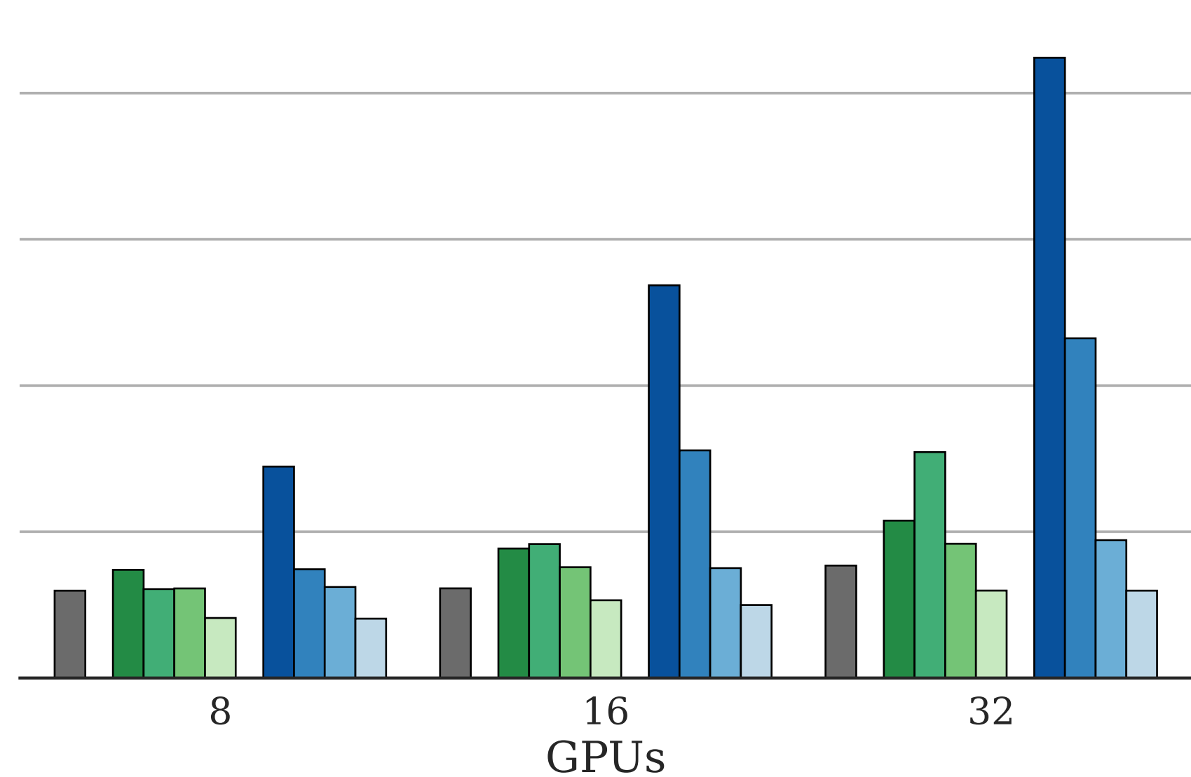
WideResNet on Polaris (NVIDIA, NCCL) - Weak Scaling Local batch 8
