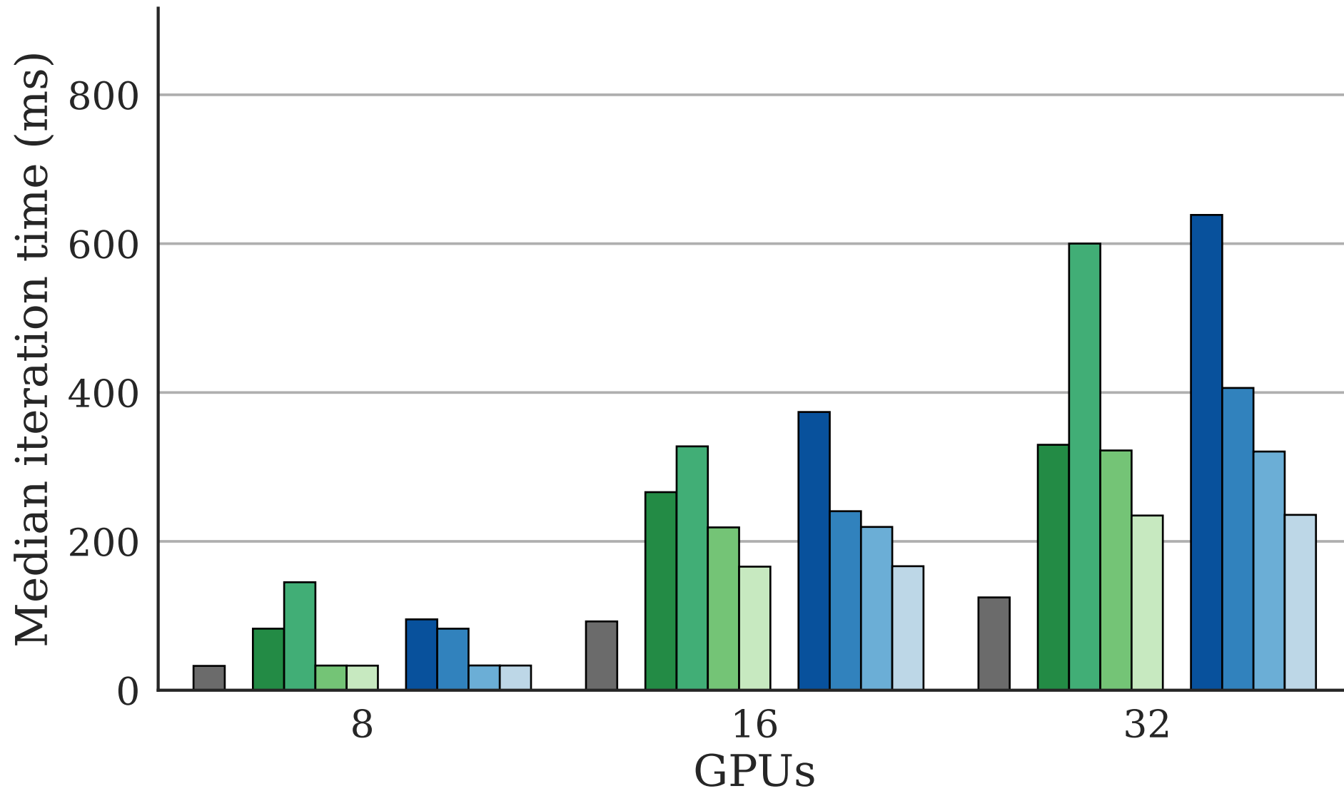
WideResNet on Frontier (AMD, RCCL) - Weak Scaling Local batch 8
