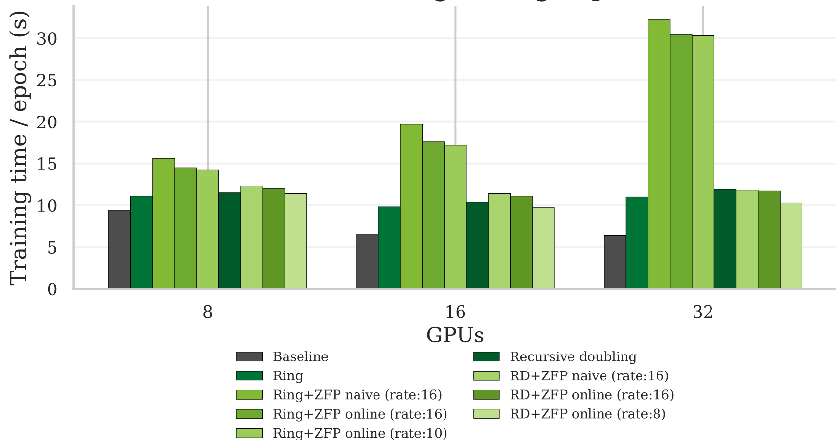
wideresnet - Strong scaling - epoch time
