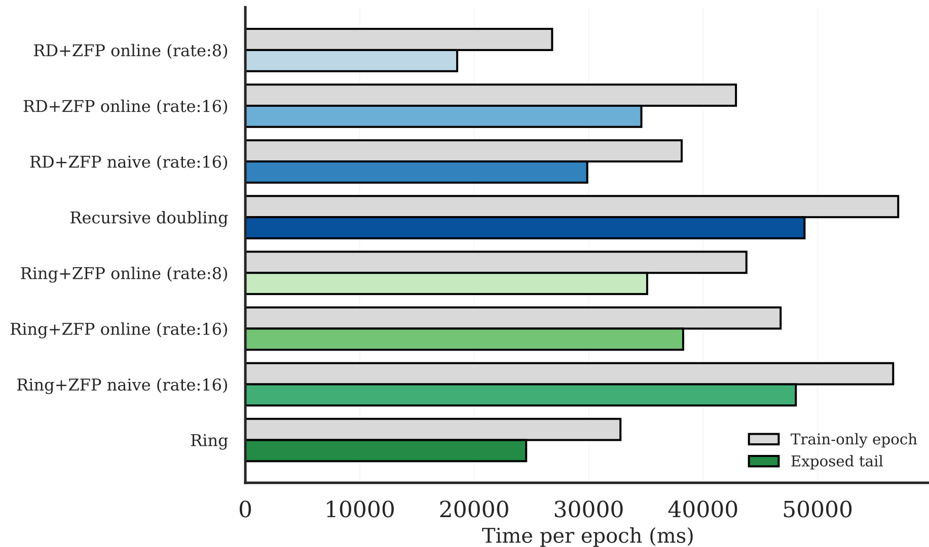
WideResNet on Polaris (NVIDIA, MPI) - Strong Scaling — Global batch 128
