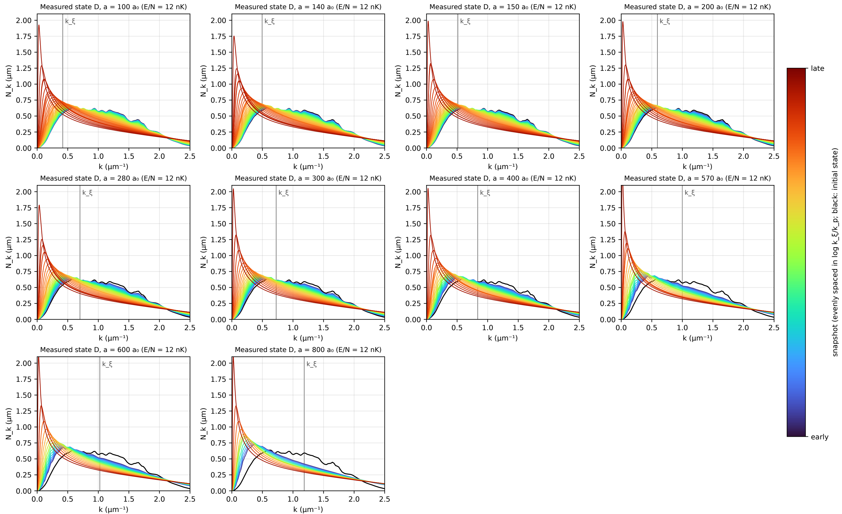
Particle spectrum N_k = 4\pi k^2 n_k / N at snapshots (Bare WKE)
