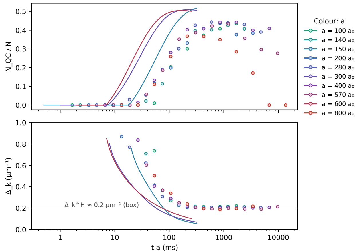
Quasi-condensate: Bubble chain, N \rightarrow \infty , Bose +1 (lines) against measured (points)
