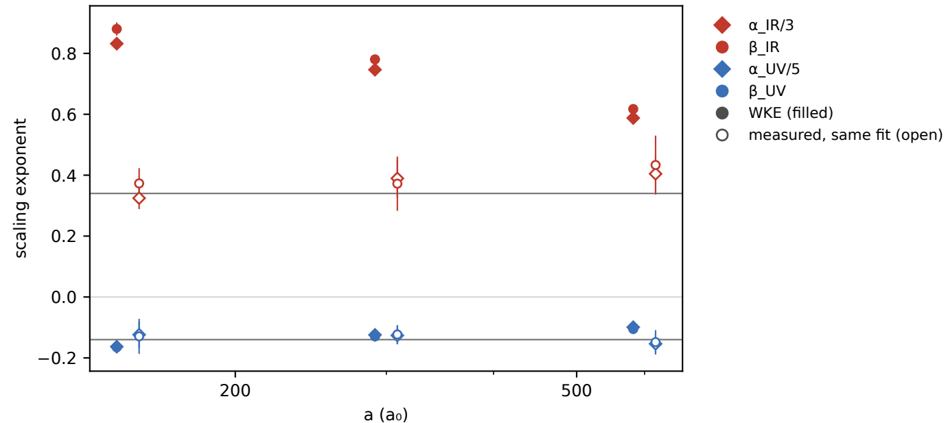
Exponents over t \bar{a} \in [20, 160] ms: Bubble chain, N \rightarrow \infty , Bose +1
