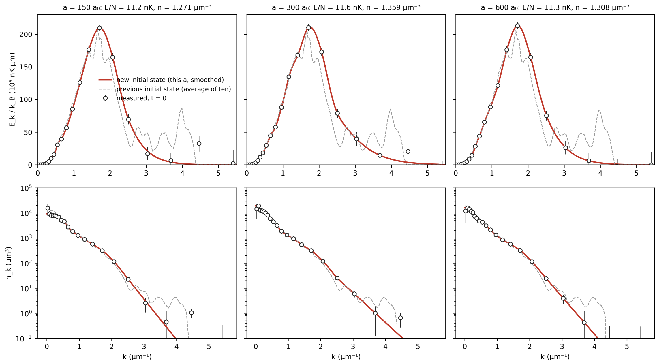
Initial frame of the large-N runs: the t = 0 spectrum measured with each a , as the solver starts from it
