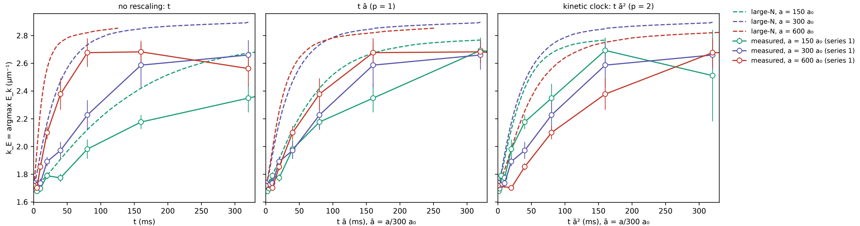
Energy peak k_E against t \bar{a}^p : large-N from each a 's own measured t = 0 state (dashed) and measured (solid)
