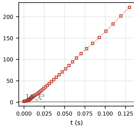
Measured state D, 600 a_0 E/N = 11 nK, a = 600 a_0
