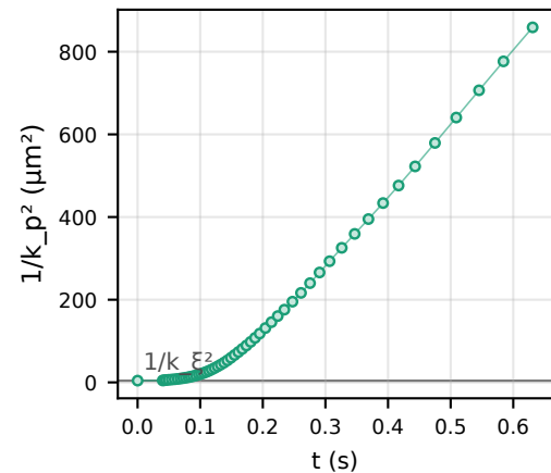
Measured state D, 150 a_0 E/N = 11 nK, a = 150 a_0
