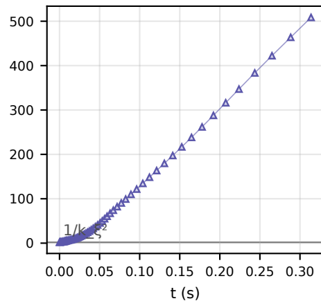
Measured state D, 300 a_0 E/N = 12 nK, a = 300 a_0
