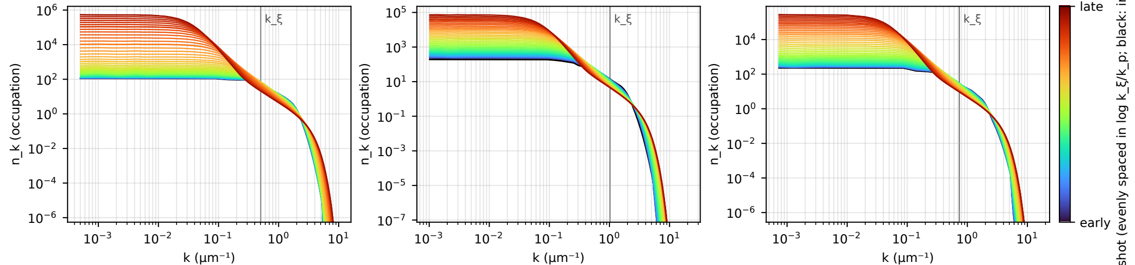
Measured state D, 150 a_0 , a = 150 a_0 ( E/N = 11 nK)
