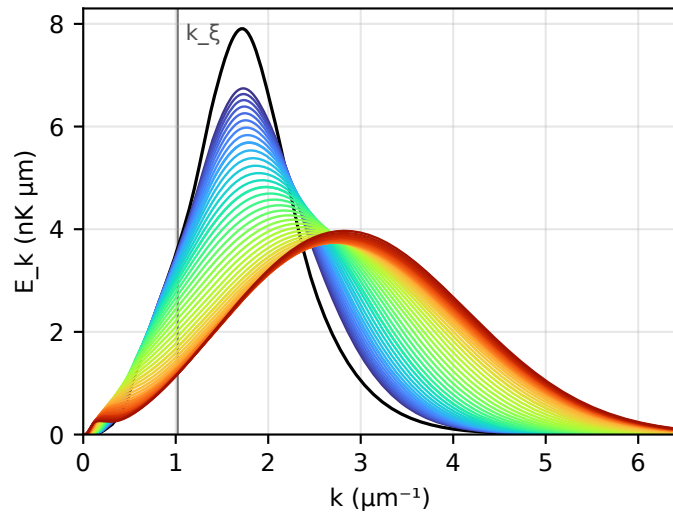
Measured state D, 600 a_0 , a = 600 a_0 ( E/N = 11 nK)
