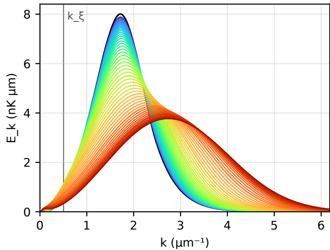
Measured state D, 150 a_0 , a = 150 a_0 ( E/N = 11 nK)
