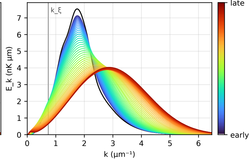
Measured state D, 300 a_0 , a = 300 a_0 ( E/N = 12 nK)
