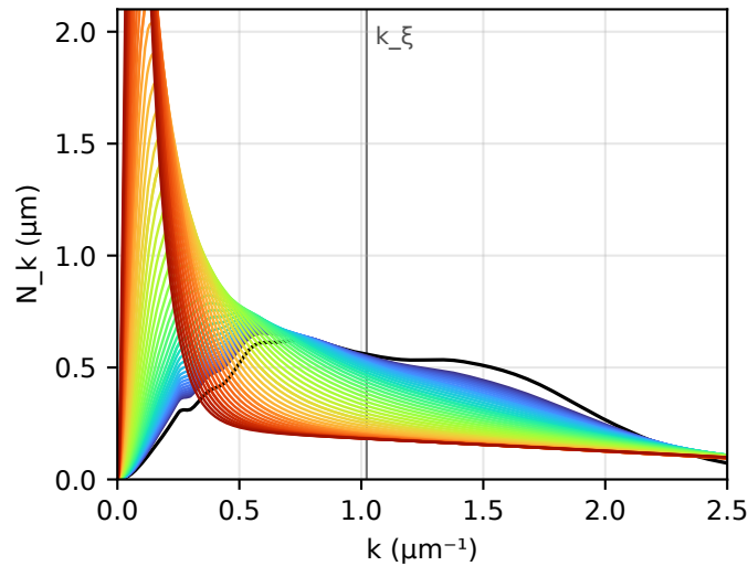
Measured state D, 600 a_0 , a = 600 a_0 ( E/N = 11 nK)
