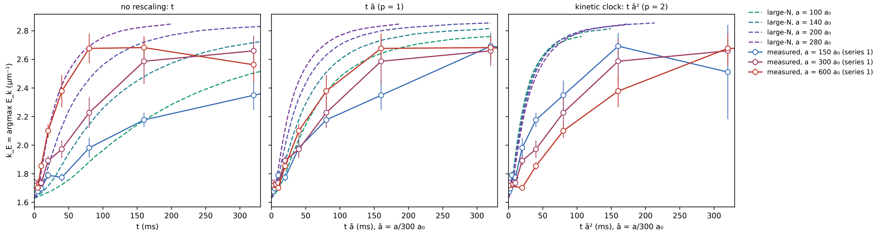
Energy peak k_E against t \bar{a}^p : large-N (dashed, bubble chain, Bose +1) and measured (solid)
