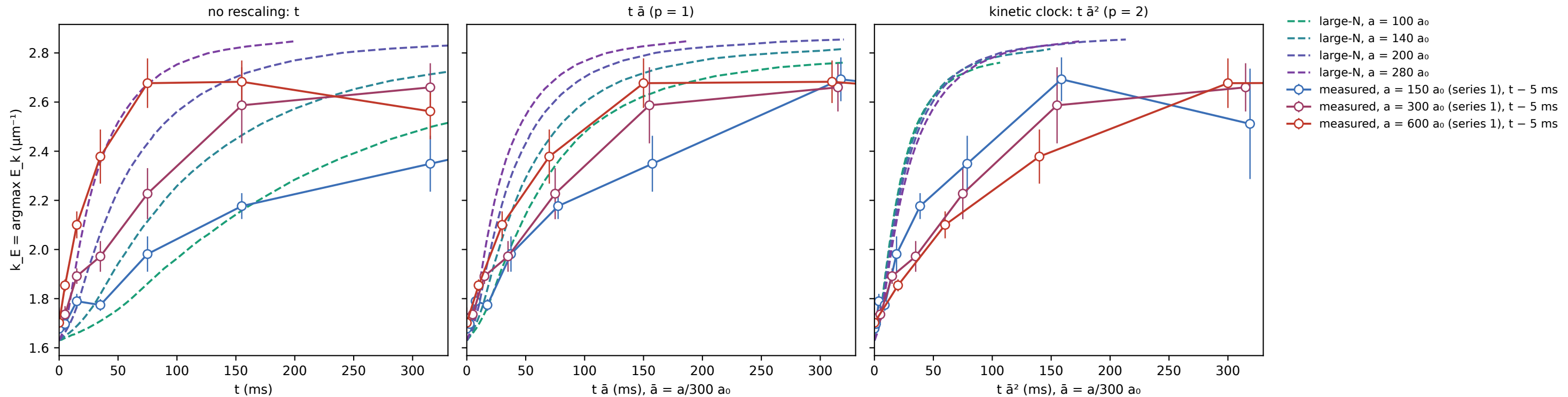
Energy peak k_E against t \bar{a}^p : large-N (dashed) and measured with t - 5 ms (solid)
