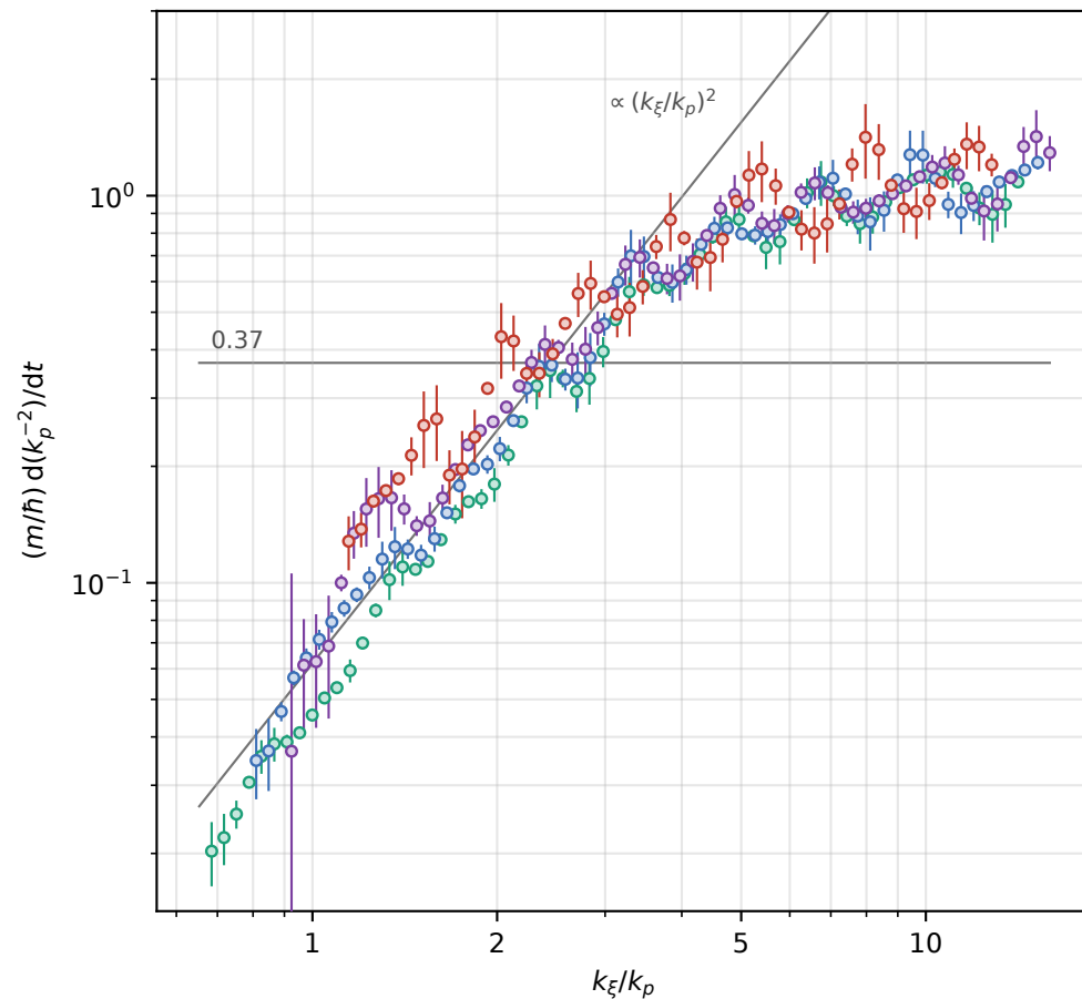
Bubble chain, N \rightarrow \infty ; standard accuracy; rate from the collision term
