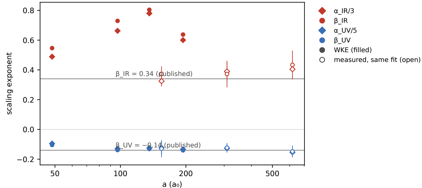
Exponents over t \bar{a} \in [20, 160] ms: Heuristic C, fitted, Bose +1
