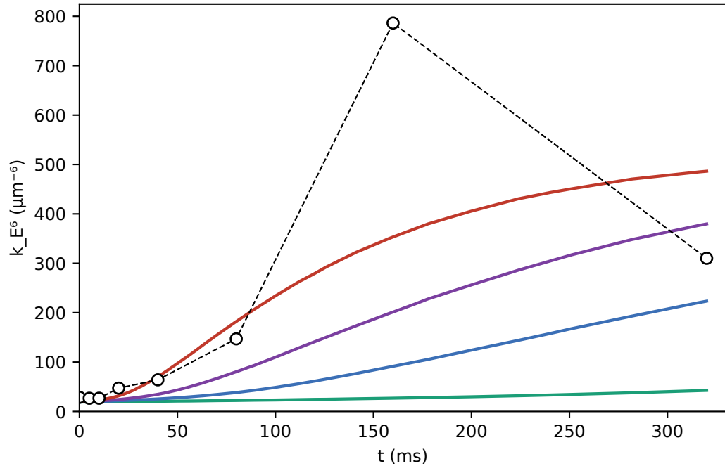
Energy peak: k_E E^6 grows linearly in t if \beta_{UV} = -1/6
