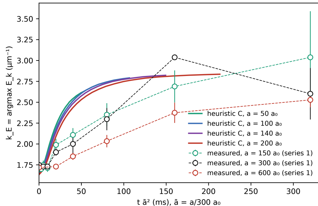
Energy peak against the kinetic clock t \bar{a}^2 : heuristic C collapses, the measured a do not
