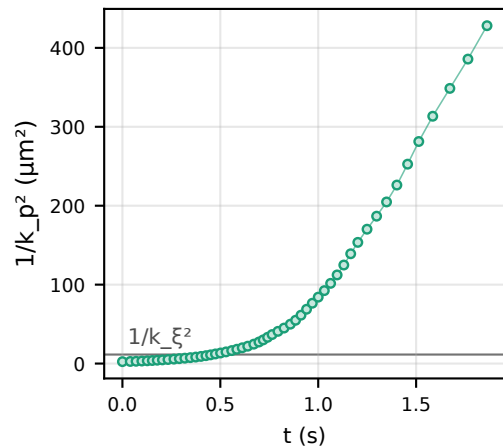
Measured state D E/N = 12 nK, a = 50 a 0
