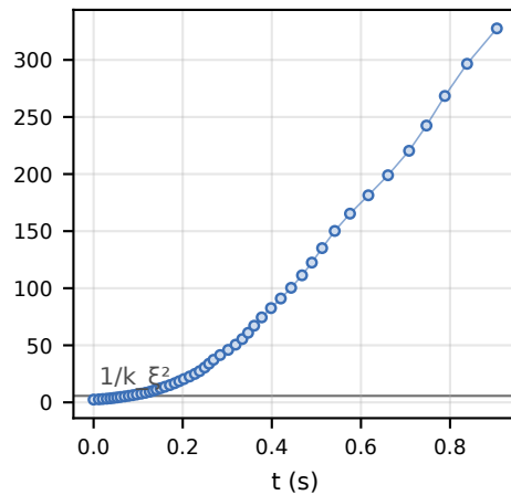
Measured state D E/N = 12 nK, a = 100 a 0
