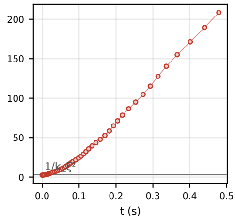
Measured state D E/N = 12 nK, a = 200 a 0
