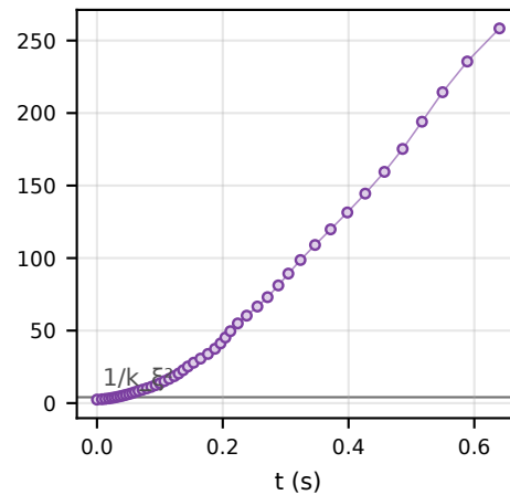
Measured state D E/N = 12 nK, a = 140 a 0
