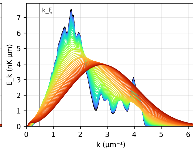
Measured state D, a = 140 a_0 ( E/N = 12 nK)
