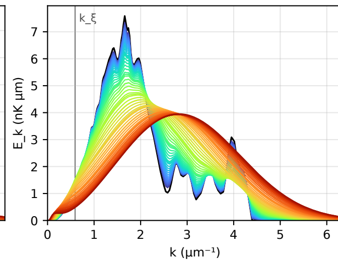
Measured state D, a = 200 a_0 ( E/N = 12 nK)
