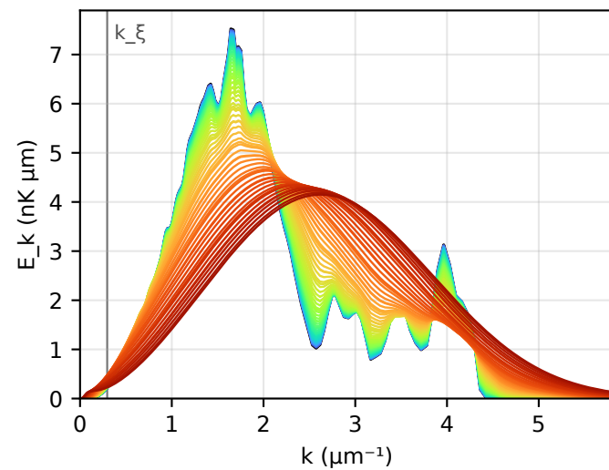
Measured state D, a = 50 a_0 ( E/N = 12 nK)
