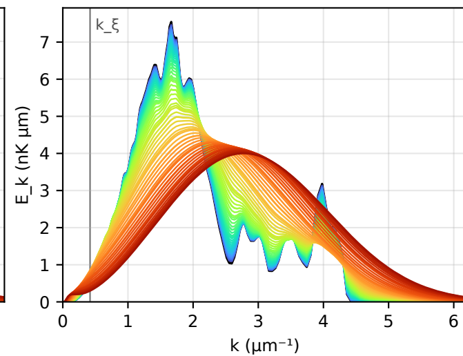
Measured state D, a = 100 a_0 ( E/N = 12 nK)
