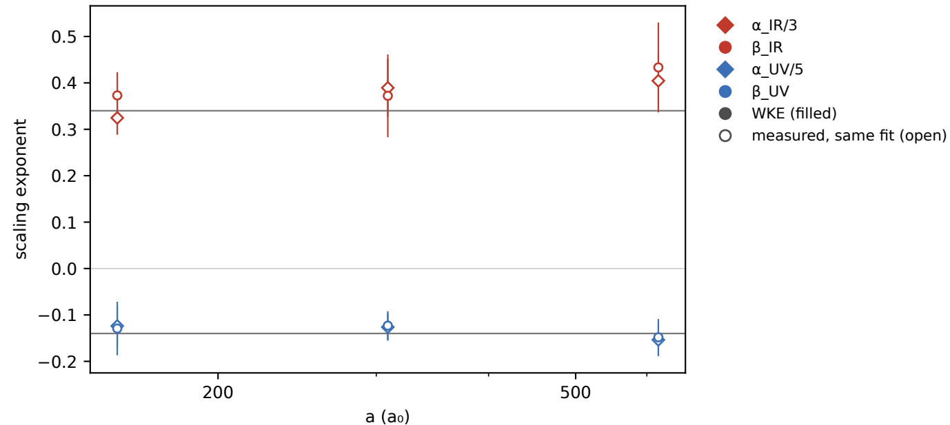
Exponents over t \bar{a} \in [20, 160] ms: One loop, N = 1 , classical
