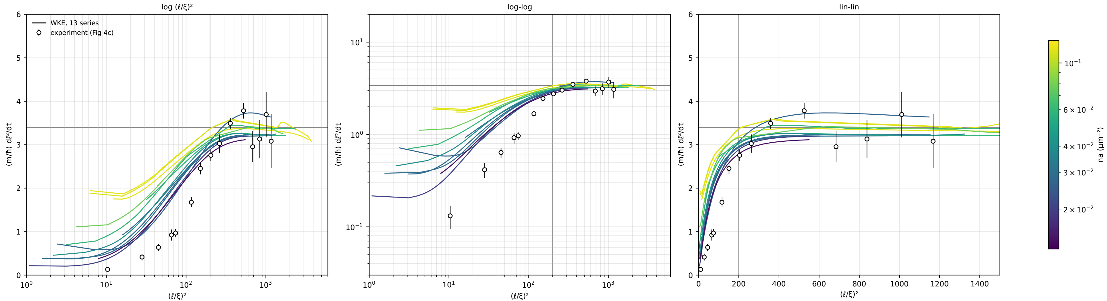
Coherence spreading rate against (\ell/\xi)^2 (Fig 4c analogue). Heuristic C, fitted, Bose +1; WKE \ell^3 = f_0/(\eta_{\text{eq}} n) ; the published \ell is deconvolved (not undone here). Guides: (\ell/\xi)^2 = 200, 3.4
