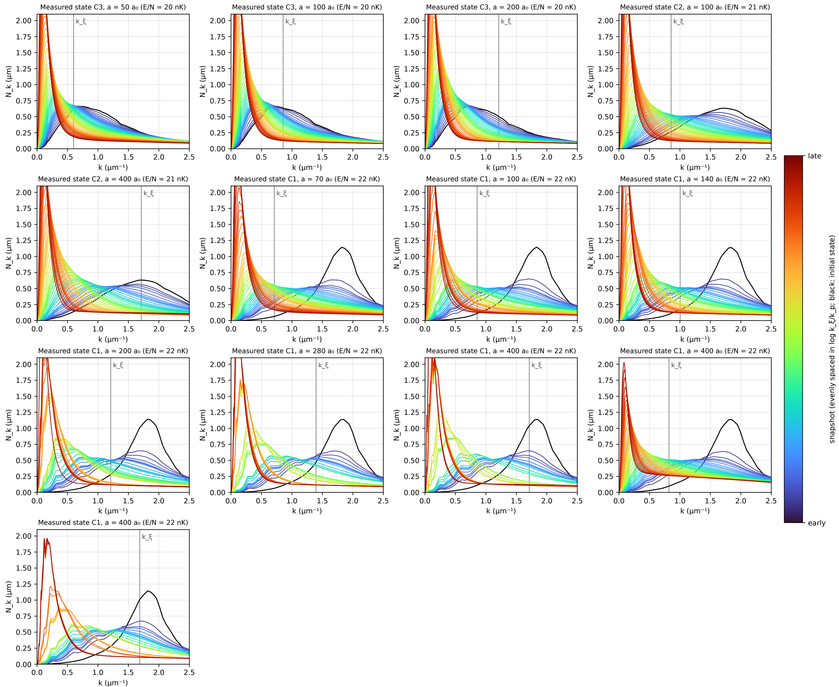
Particle spectrum N_k = 4\pi k^2 n_k / N at snapshots (Heuristic C, fitted)
