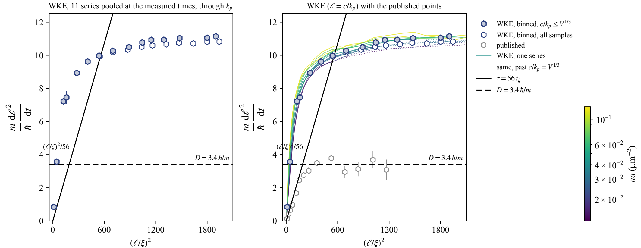
Fig 4c analogue. WKE Bubble chain, N \rightarrow \infty , Bose +1, standard; WKE through k_p : \ell = c/k_p , k_p the peak of N_k \propto k^2 n_k ; c = 3.09 \pm 0.03 from the WKE alone ( \ell^2 = c^2/k_p^2 , (\ell/\xi)^2 \geq 200 )
