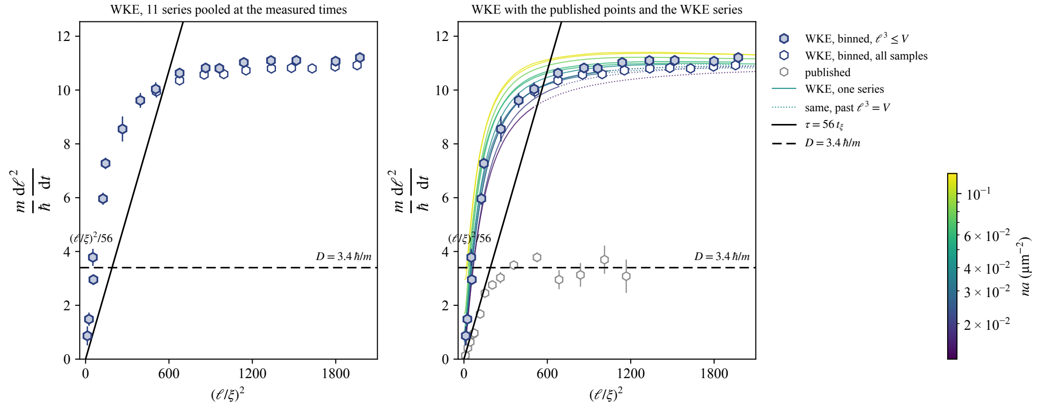
Fig 4c analogue. WKE Bubble chain, N \rightarrow \infty , Bose +1, standard; \ell^3 = f_0/(\eta_{\text{eq}} n) ; the published \ell carries a deconvolution that is not undone
