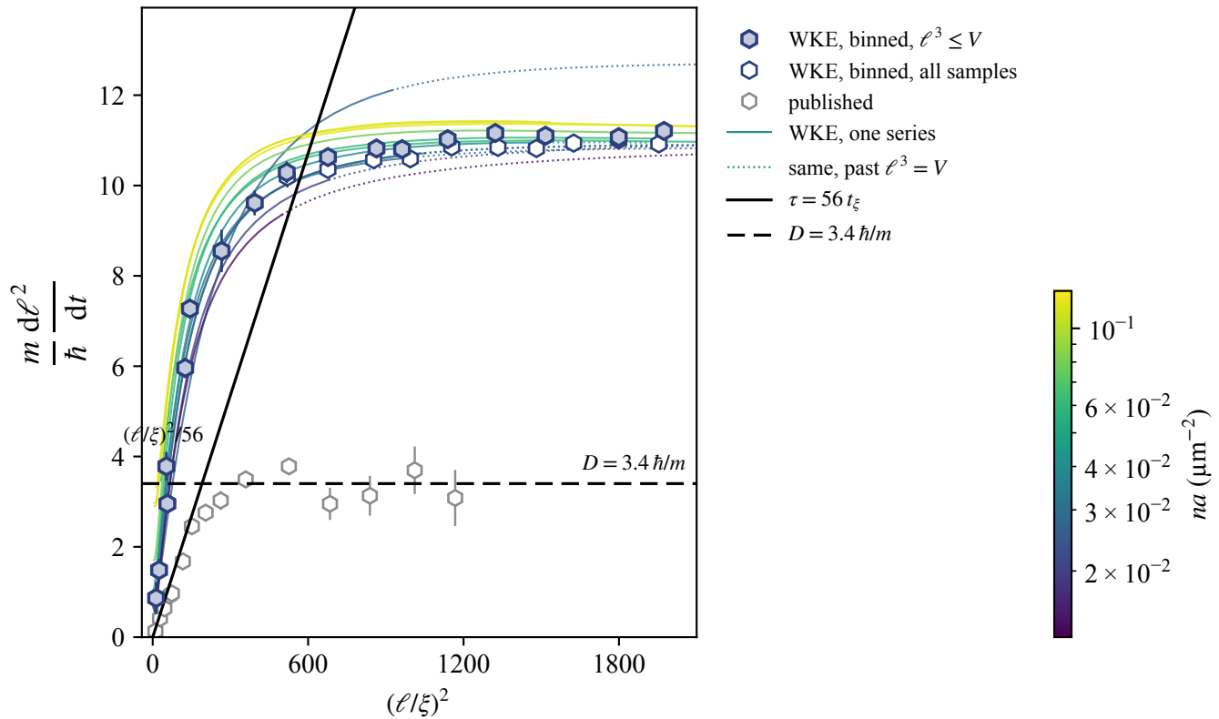
Fig 4c analogue. WKE Bubble chain, N \rightarrow \infty , Bose +1, standard; \ell^3 = f_0/(\eta_{\text{eq}} n) ; the published \ell carries a deconvolution that is not undone
