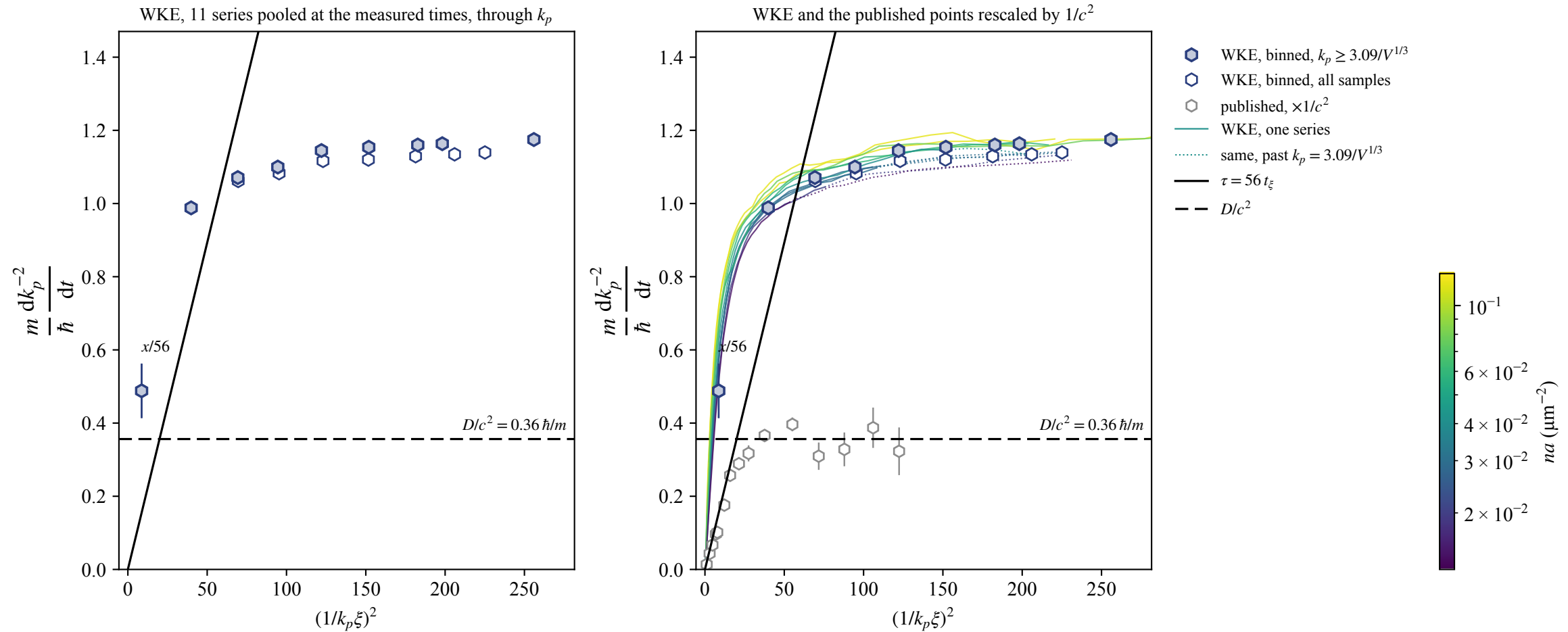
Fig 4c analogue. WKE Bubble chain, N \rightarrow \infty , Bose +1, standard; k_p the peak of N_k \propto k^2 n_k ; published points and D rescaled by 1/c^2 , c = 3.09 \pm 0.03 from the WKE alone ( \ell^2 = c^2/k_p^2 , (\ell/\xi)^2 \geq 200 )
