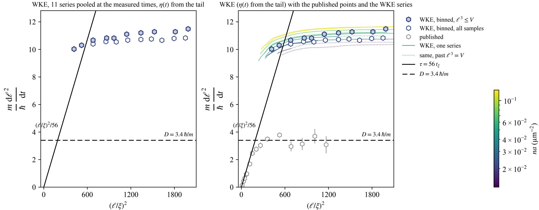
Fig 4c analogue. WKE Bubble chain, N \rightarrow \infty , Bose +1, standard; \ell^3 = f_0/(\eta(t) n(t)) , \eta(t) from a \mu = 0 Bose-Einstein fit of the thermal tail ( 0.05 < f < 5 ) at every snapshot; the published \ell carries a deconvolution that is not undone
