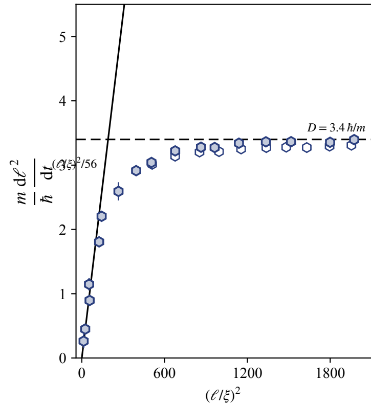
Fig 4c analogue. WKE Bubble chain, N \rightarrow \infty , Bose +1, standard; \ell^3 = f_0/(\eta_{\text{eq}} n) ; the published \ell carries a deconvolution that is not undone; WKE rates divided by 3.3
