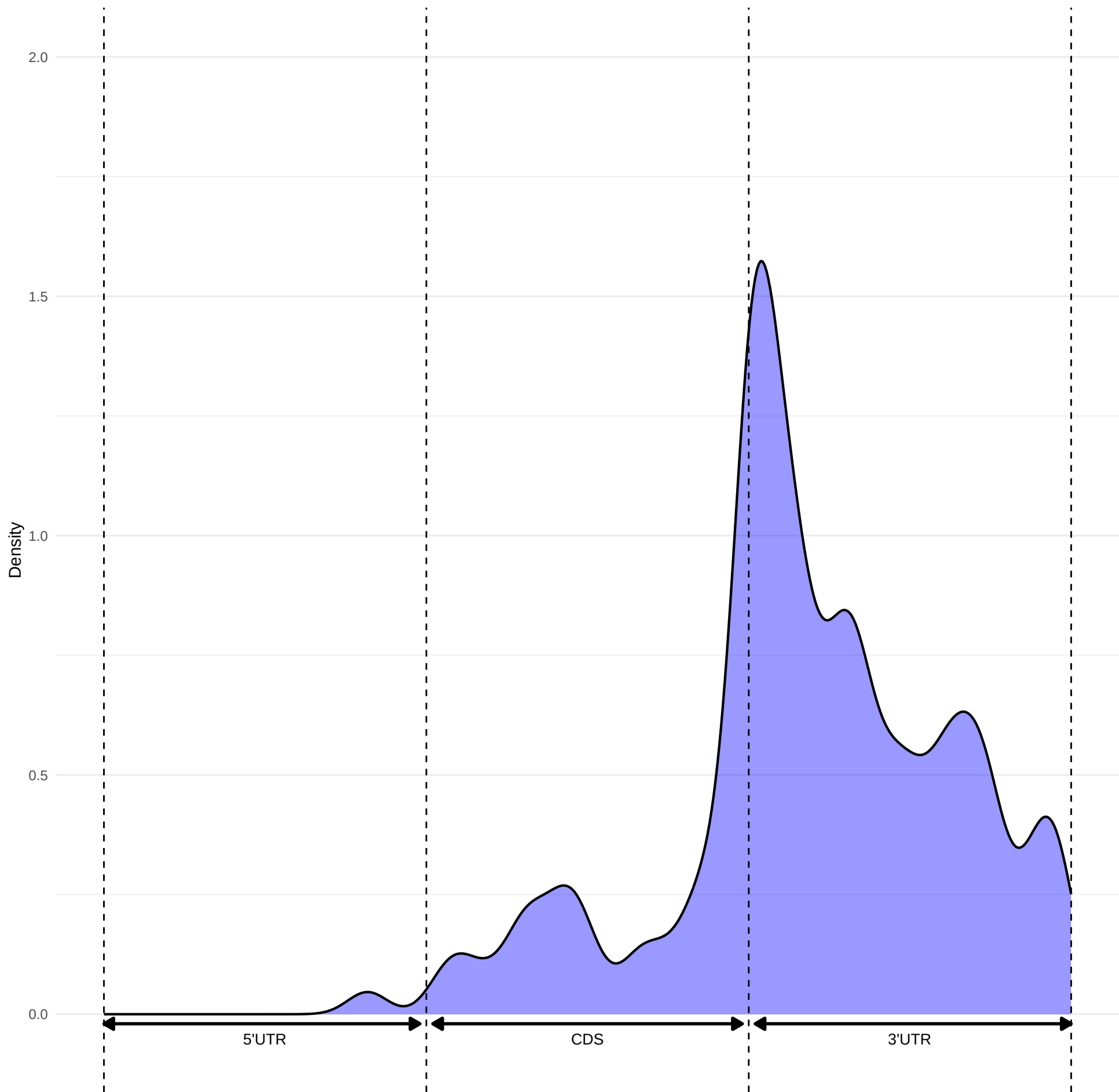
Transcriptome-wide m6A Distribution for: naive
